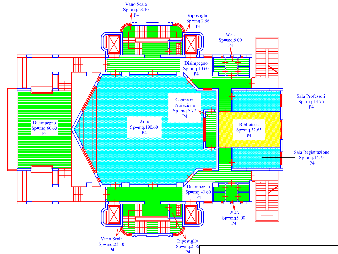
Piano Quarto H=mt.3.70
