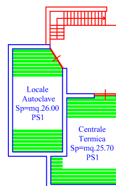
Piano Seminterrato H=mt.3.30
